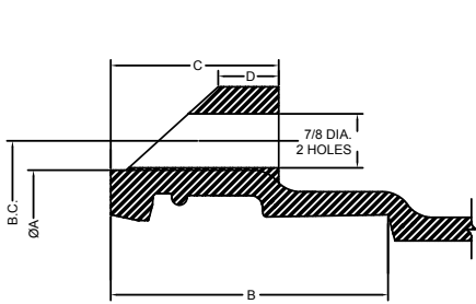
4"-12" SIZES
